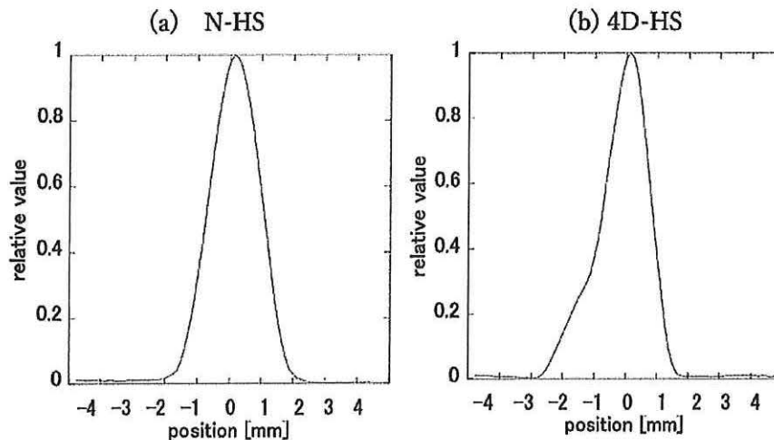
Fig. 2. Results of slice sensitivity profile (SSP) with QUASAR respiratory synchronous phantom (RM Phantom) under situation 1. The x-axis represents the body-axis direction, and the y-axis represents the computed tomography (CT) value of the coin phantom as a relative value.
