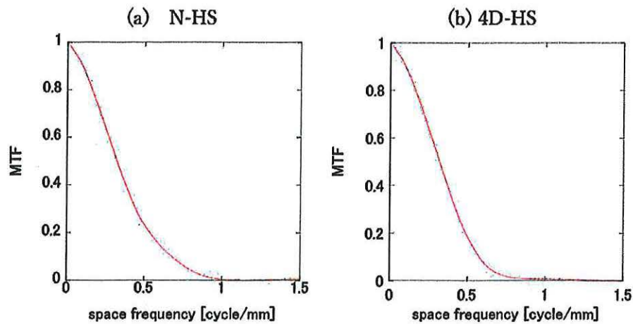
Fig. 11. Modulation transfer function (MTF) results with the RM Phantom under situation 1. The x-axis represents the space frequency, and the y-axis represents the MTF.
