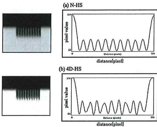
Fig. 6. Images and profiles with multiplanar reconstruction profile (MPR) with a slit width of 0.6 mm. The sagittal plane of MPR and its profile are shown. a : Result for normal helical scanning (N-HS). b : Result for respiratory-gated helical scan four-dimensional system (4D-HS).
