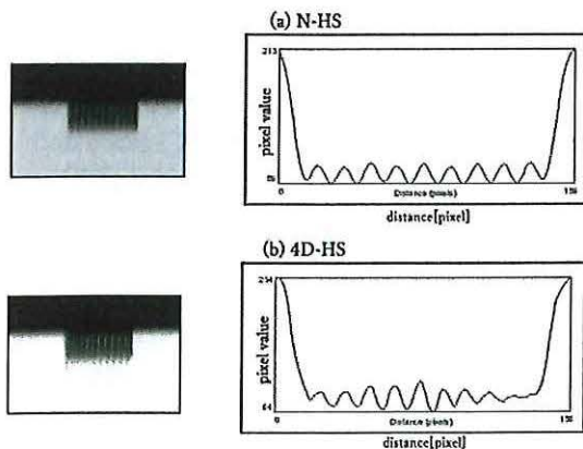
Fig. 7. Images and profiles with multiplanar reconstruction profile (MPR) with a slit width of 0.5 mm. The sagittal plane of MPR and its profile are shown. a : Result for normal helical scanning (N-HS). b : Result for respiratory-gated helical scan four-dimensional system (4D-HS).
